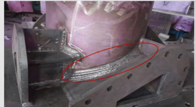
Multi layer and multi pass welding of intersecting line welds with a 30 degree climbing slope
